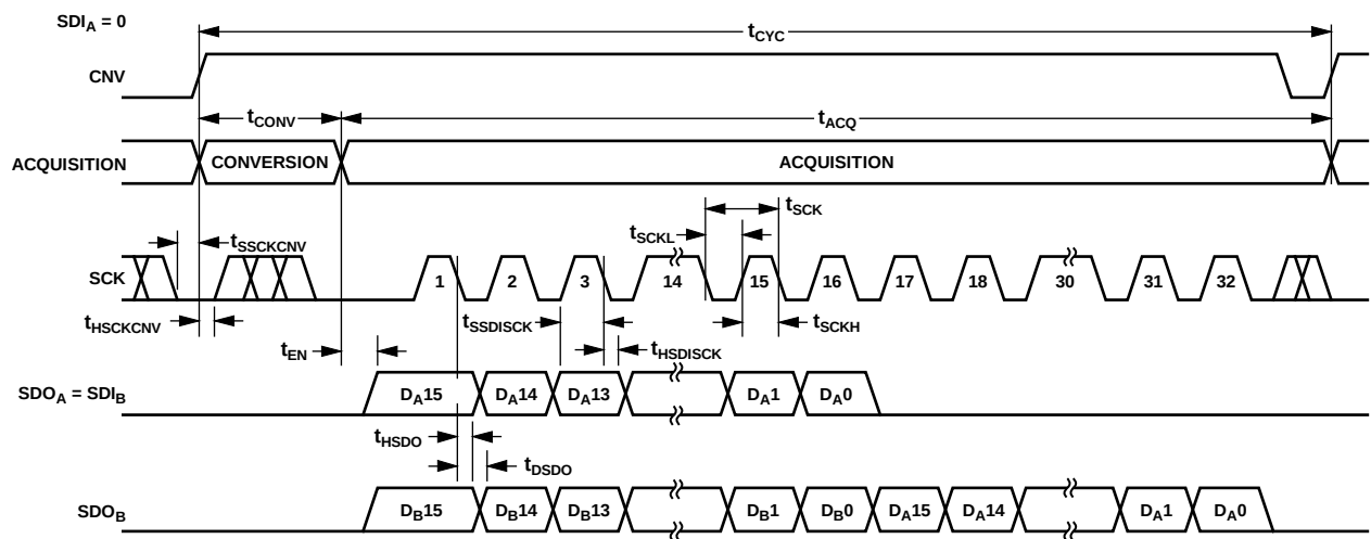
Figure 39. Chain Mode Serial Interface Timing
