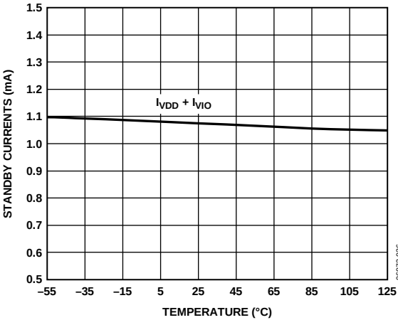
Figure 19. Standby Currents vs. Temperature
