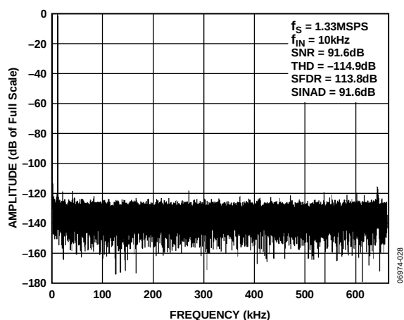
Figure 7. FFT Plot
