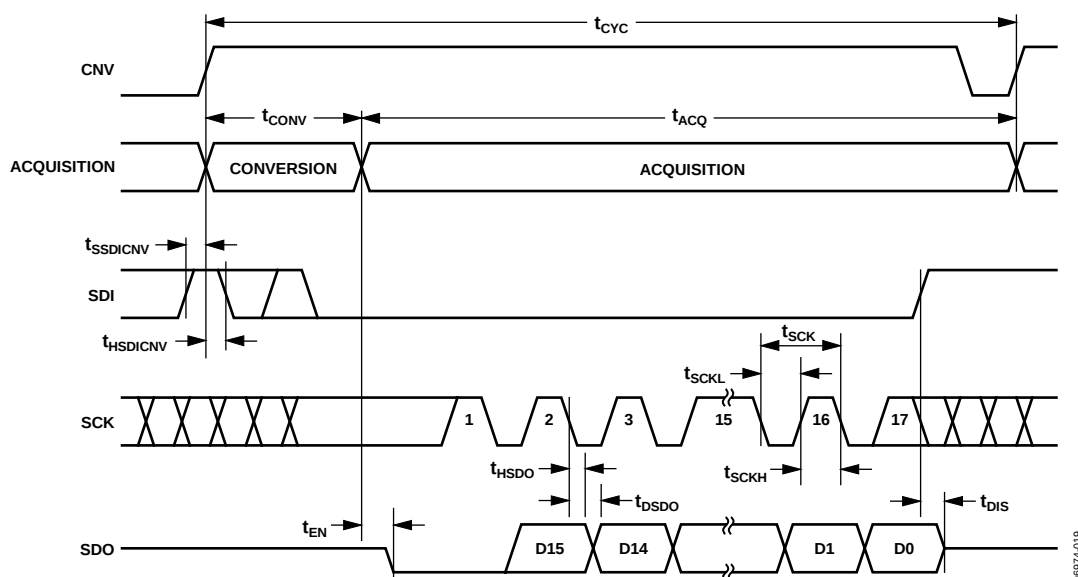
Figure 32. \overline{\text{CS}} Mode, 4-Wire with Busy Indicator Serial Interface Timing
