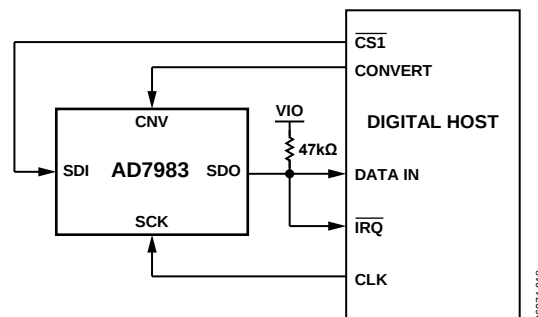
Figure 31. \overline{\text{CS}} Mode, 4-Wire with Busy Indicator Connection Diagram
