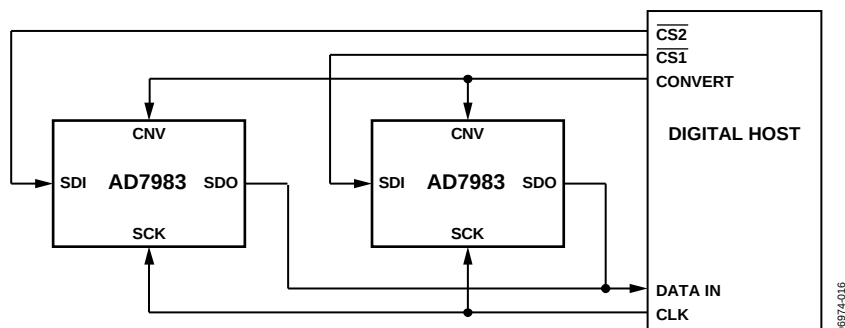
Figure 29. \overline{\text{CS}} Mode, 4-Wire Without Busy Indicator Connection Diagram
