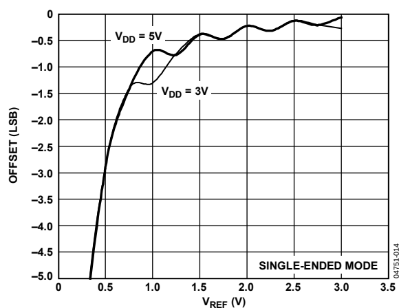
Figure 12. AD7938-6 Offset vs. V_{REF}
