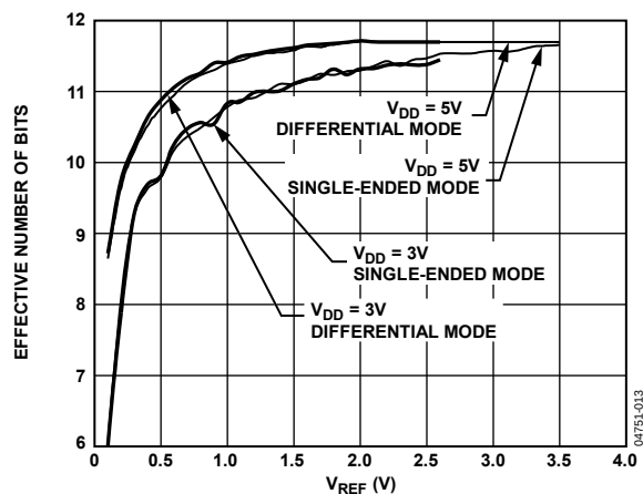
Figure 11. AD7938-6 ENOB vs. V_{REF}
