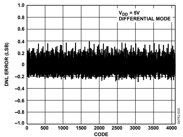
Figure 8. AD7938-6 Typical DNL at V_{DD} = 5\text{V}
