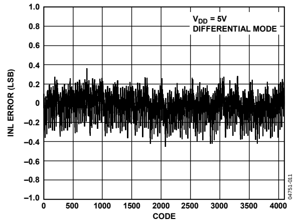
Figure 9. AD7938-6 Typical INL at V_{DD} = 5\text{V}
