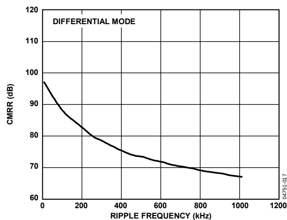
Figure 14. CMRR vs. Input Frequency with V_{DD} = 5\text{ V} and 3\text{ V}
