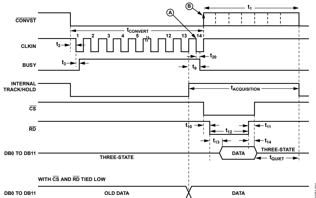
Figure 36. AD7938-6 Parallel Interface—Conversion and Read Cycle Timing in Word Mode (W/B = 1)
