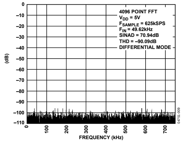
Figure 7. AD7938-6 FFT at V_{DD} = 5\text{V}
