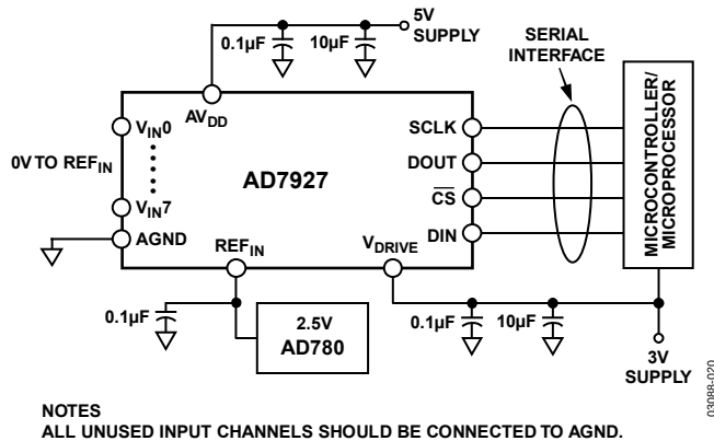
Figure 20. Typical Connection Diagram
