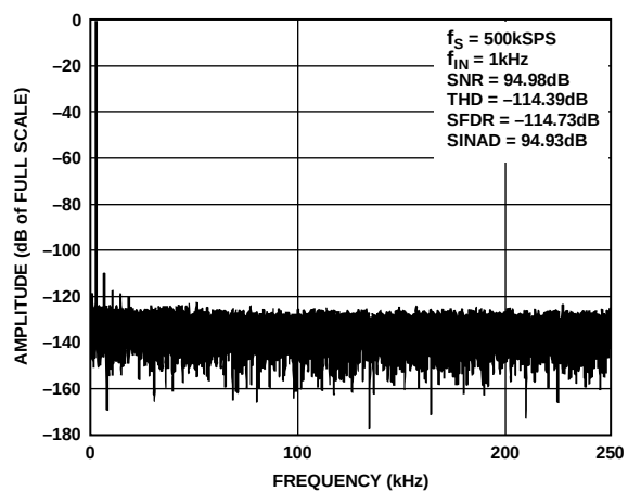
Figure 7. AD7916 FFT Plot, REF = 5 V
