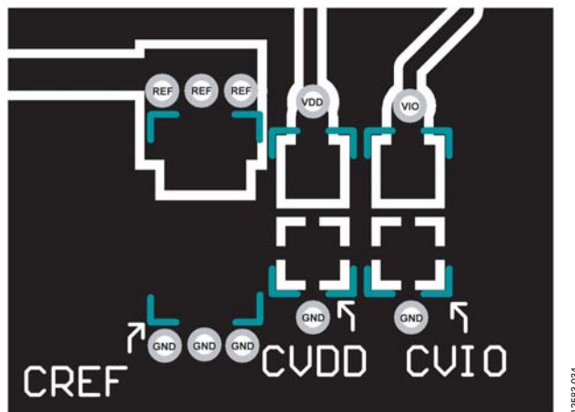
Figure 50. Recommended Layout of the AD7915/AD7916 (Bottom Layer)
