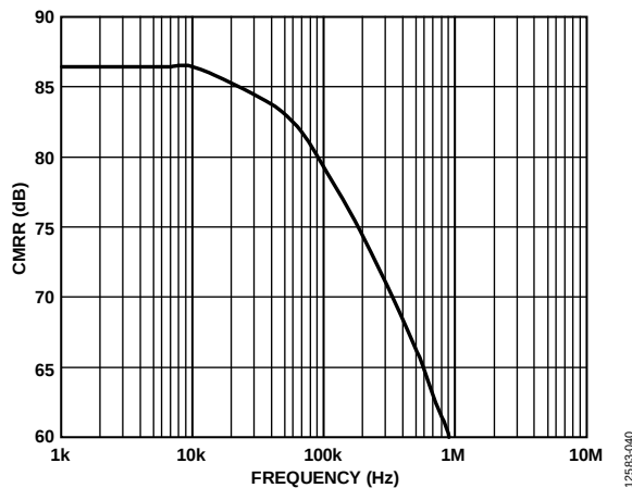
Figure 32. Analog Input CMRR vs. Frequency
