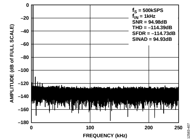
Figure 7. AD7916 FFT Plot, REF = 5 V
