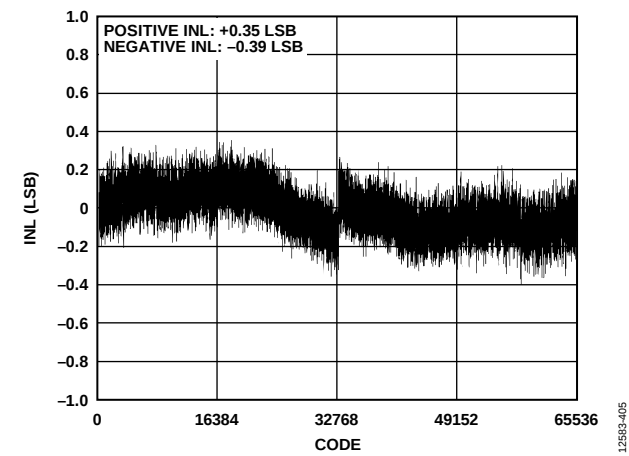
Figure 5. Integral Nonlinearity (INL) vs. Code, REF = 5 V
