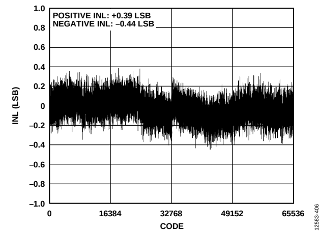
Figure 6. INL vs. Code, REF = 2.5 V
