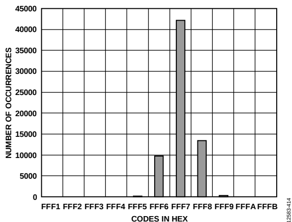
Figure 13. Histogram of a DC Input at the Code Center, REF = 2.5 V
