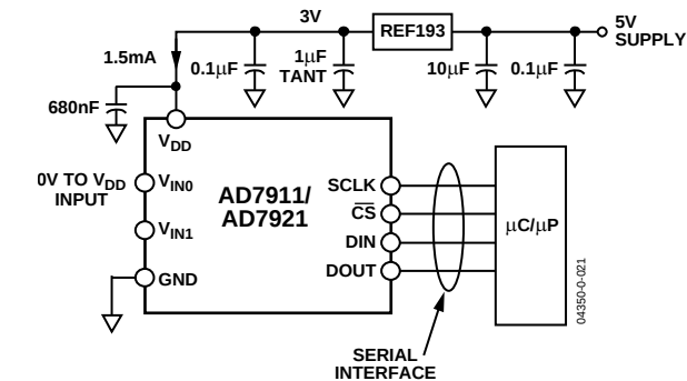
Figure 22. REF193 as Power Supply to AD7911/AD7921
