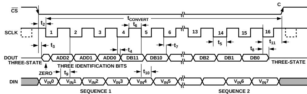
Figure 30. AD7928 Writing to SHADOW Register Timing Diagram
