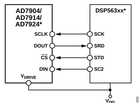
Figure 32. Interfacing to the DSP563xx
