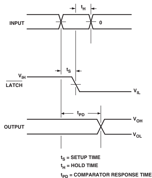
Figure 4. Latch Timing
