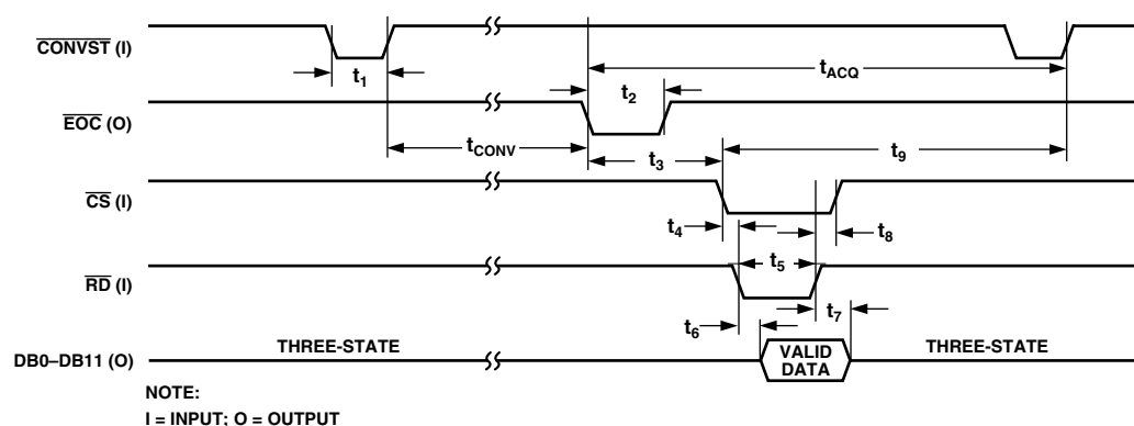
Figure 2. Parallel Mode Timing Diagram
