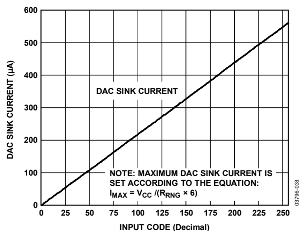
Figure 25. DAC Sink Current vs. Input Code with R RNG = 1 kΩ
