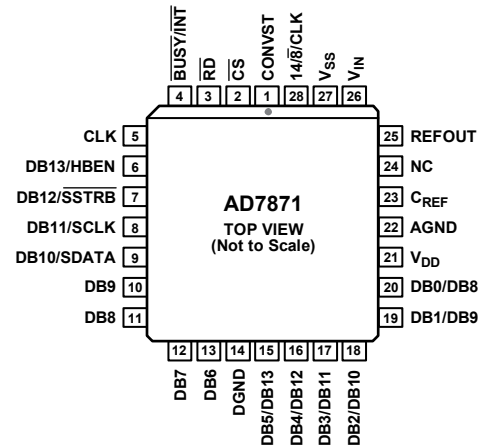
Figure 7. AD7871 PLCC
