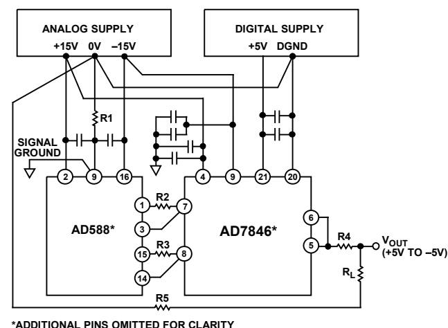
Figure 30. AD7846 Grounding
