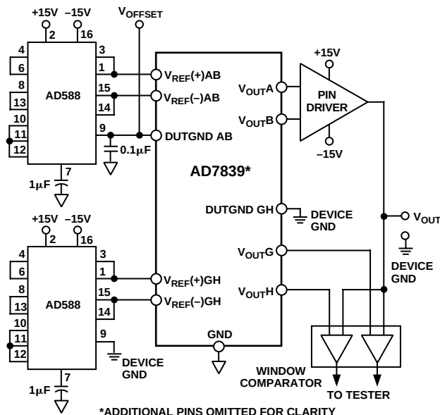
Figure 21. ATE Application
