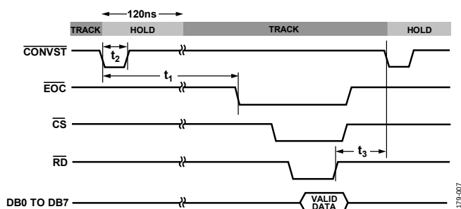
Figure 6. Track-and-Hold Timing
