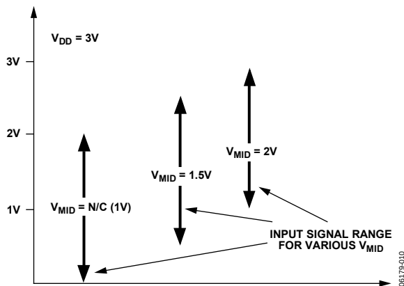
Figure 9. Analog Input Span Variation with V_{MID}
