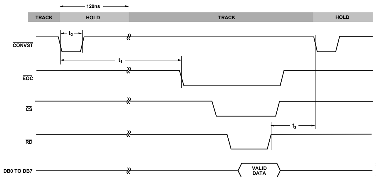
Figure 21. Mode 1 Operation
