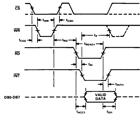
Figure 12b. \overline{WR} - \overline{RD} Mode ( t_{RD} < t_{INTL} )
