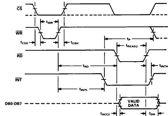
Figure 12a. \overline{WR} - \overline{RD} Mode ( t_{RD} > t_{INTL} )
