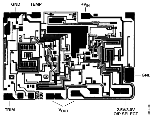
Figure 3. Die Layout
