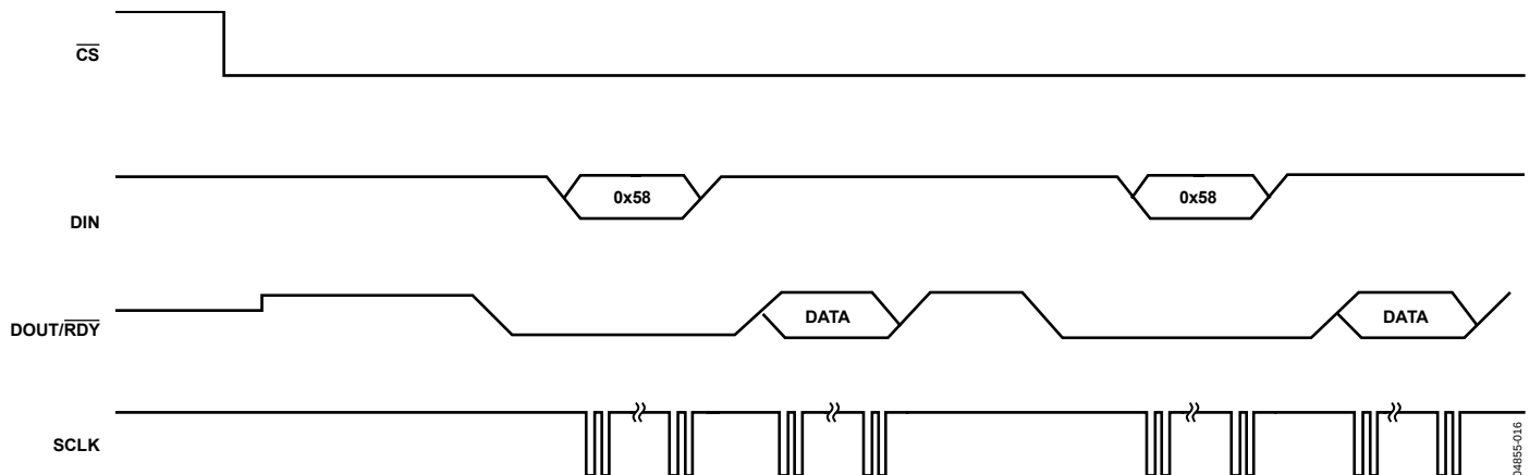
Figure 18. Continuous Conversion
