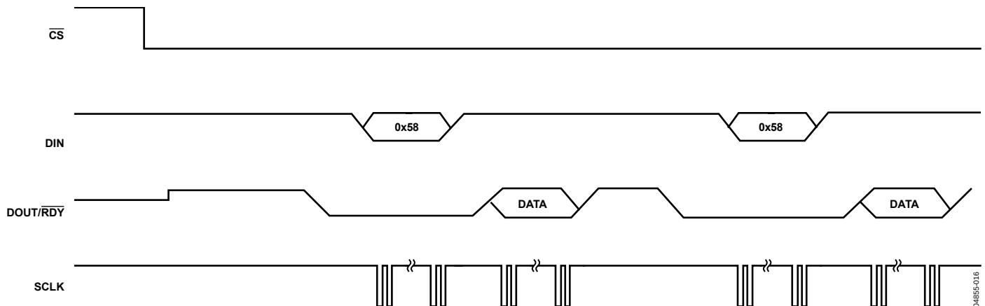
Figure 18. Continuous Conversion
