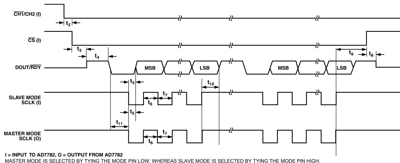
Figure 2. Slave/Master Mode Timing Diagram
