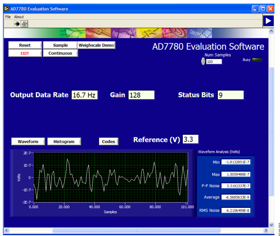
Figure 3. AD7780 Evaluation Software Main Window
