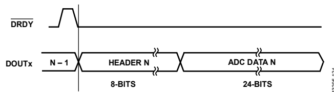
Figure 107. ADC Output—8-Bit Header + 24-Bit Conversion Data
