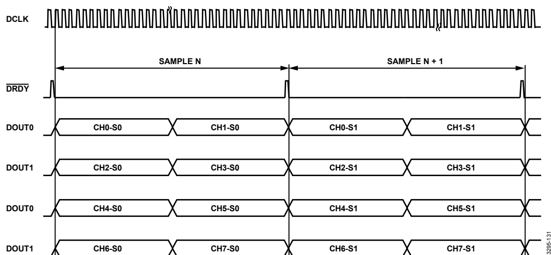
Figure 117. FORMAT0 = 0 , FORMAT1 = 0 —Each DOUTx Outputs Two ADC Conversions (S0 Means Sample 0 and S1 Means Sample 1)
