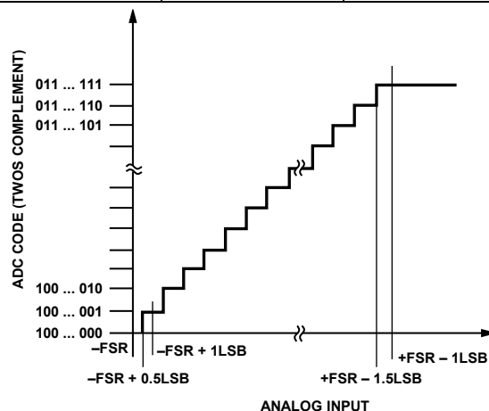
Figure 90. Transfer Function
