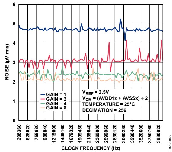
Figure 24. Noise vs. Clock Frequency at 2 kSPS, Low Power Mode, Decimation = 256
