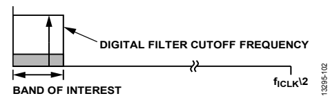
Figure 84. \Sigma - \Delta ADC Operation, Removal of Noise Energy from the Band of Interest (Linear Scale X-Axis)
