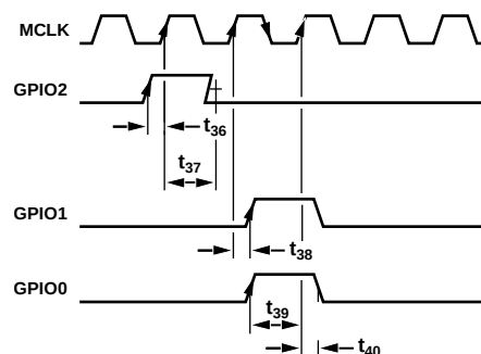
Figure 6. GPIOs for SRC Update Timing Diagram
