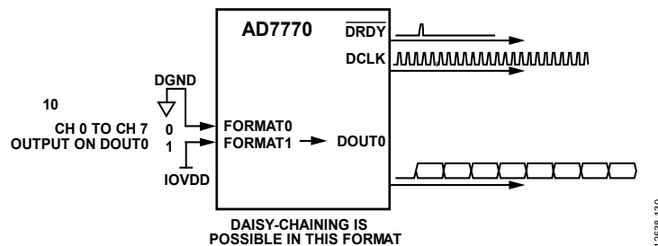
Figure 115. FORMATx Pin Configuration—FORMAT0 = 0, FORMAT1 = 1
