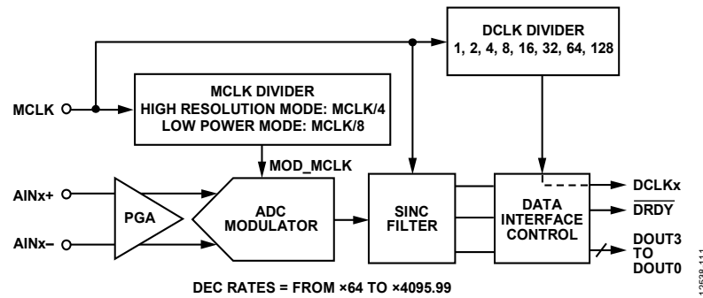
Figure 94. Clock Generation on the AD7770
