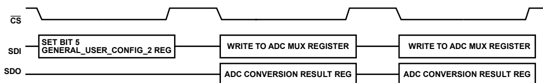
Figure 106. Configuring the AD7770 to Operate the SPI to Read from the SAR ADC
