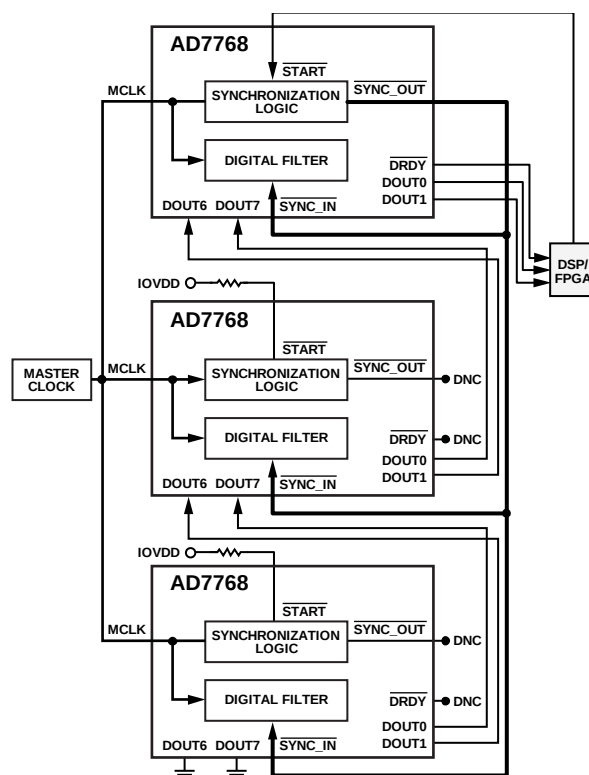
Figure 104. Daisy-Chaining Multiple AD7768 Devices
