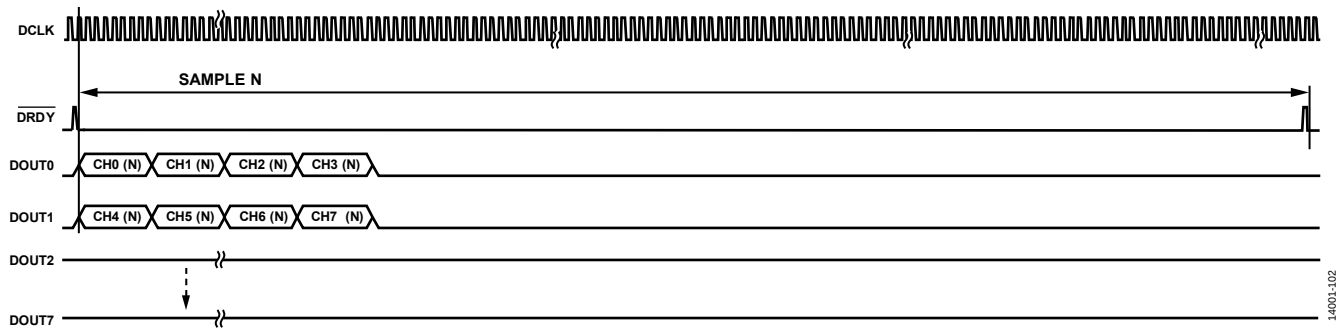
Figure 102. AD7768 \text{FORMATx} = 01 : Channel 0 to Channel 3 Share DOUT0, and Channel 4 to Channel 7 Share DOUT1, Decimation=512
