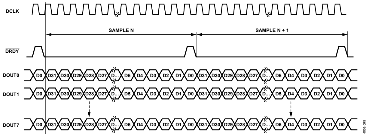
Figure 100. AD7768 \text{FORMATx} = 00 : Each ADC Has a Dedicated Data Output Pin, Maximum Data Rate
