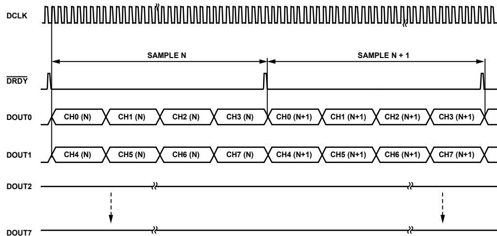
Figure 101. AD7768 \text{FORMATx} = 01 : Channel 0 to Channel 3 Share DOUT0, and Channel 4 to Channel 7 Share DOUT1, Maximum Data Rate
