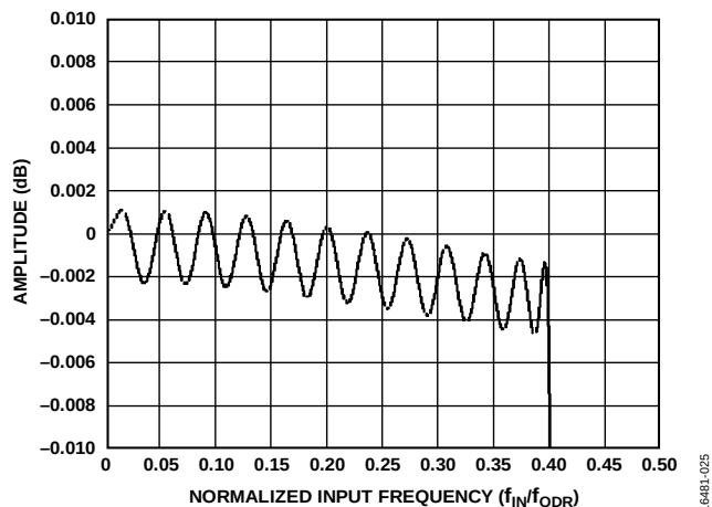
Figure 74. Low Ripple FIR Filter Pass-Band Ripple
