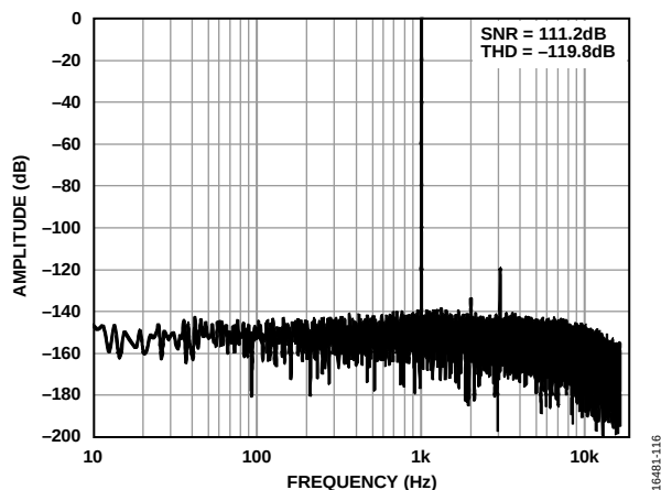
Figure 15. FFT, Low Power Mode, Sinc5 Filter, -0.25 dBFS
