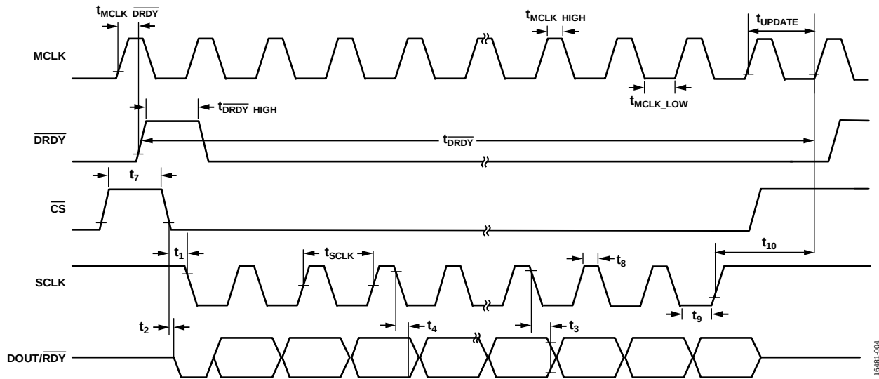
Figure 4. Reading Conversion Result in Continuous Conversion Mode ( \overline{CS} Toggling)
