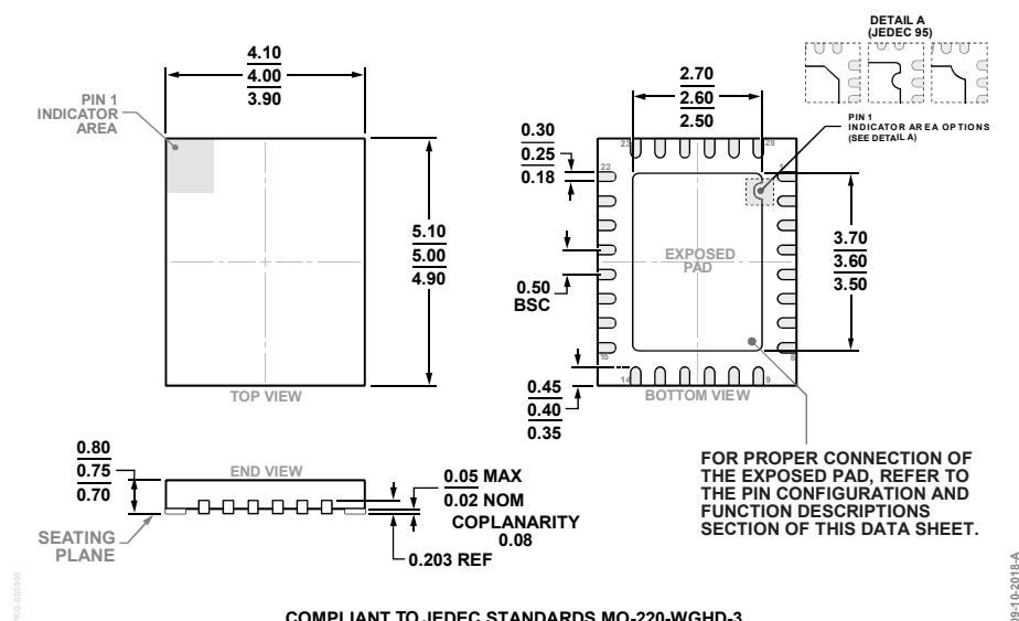
COMPLIANT TO JEDEC STANDARDS MO-220-WGHD-3 Figure 101. 28-Lead Lead Frame Chip-Scale Package [LFCSP] 4 mm x 5 mm Body and 0.75 mm Package Height (CP-28-12) Dimensions shown in millimeters
