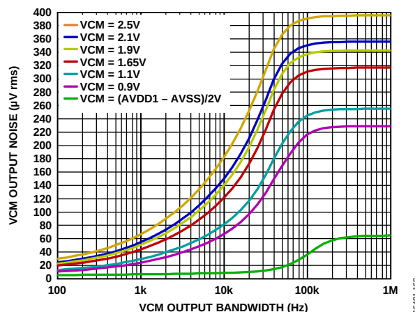
Figure 66. VCM Output Noise vs. VCM Output Bandwidth
