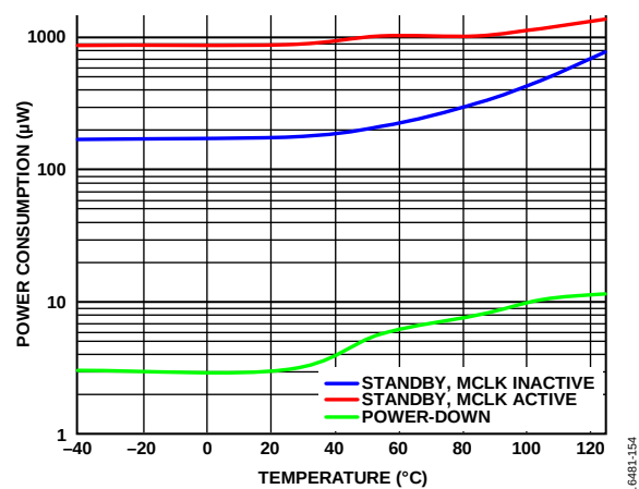
Figure 52. Power Consumption, Standby and Power-Down vs. Temperature, \text{AVDD1}, \text{AVDD2} = 5\text{ V} , \text{IOVDD} = 1.8\text{ V}
