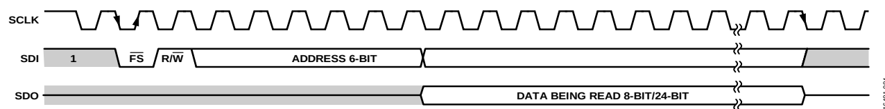
Figure 88. 3-Wire SPI Read Frame ( \overline{\text{CS}} = 0 )
