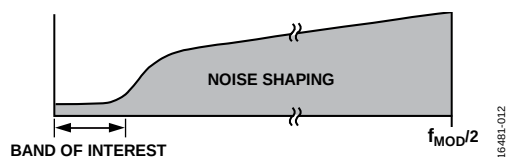
Figure 58. \Sigma - \Delta ADC Noise Shaping (Linear Scale X-Axis)
