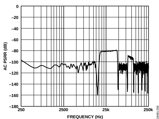
Figure 56. AVDD1 AC PSRR vs. Frequency, Low Power Mode, \text{AVDD1} = 5\text{ V} + 0.1\text{ V p-p}
