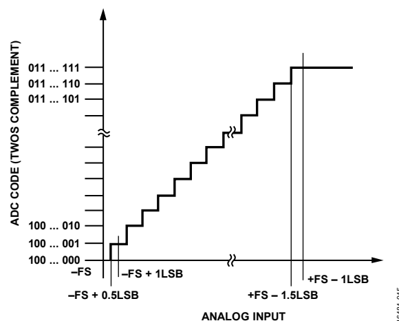
Figure 61. ADC Ideal Transfer Functions (FS is Full-Scale)
