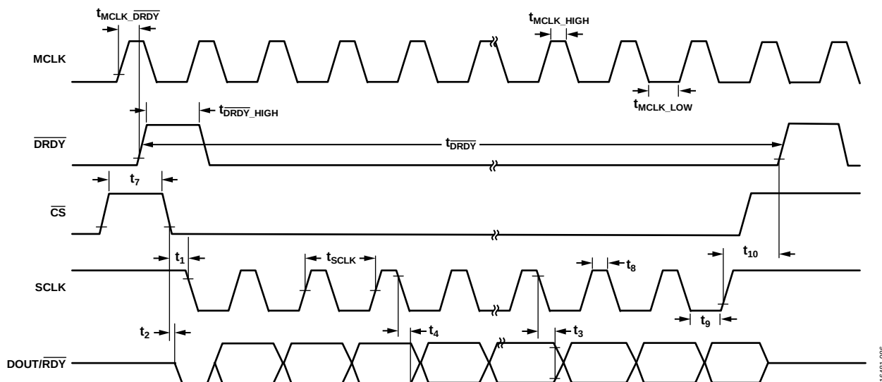
Figure 90. Serial Interface Timing Diagram, Example Reflects Reading an ADC Conversion in Continuous Read Mode
