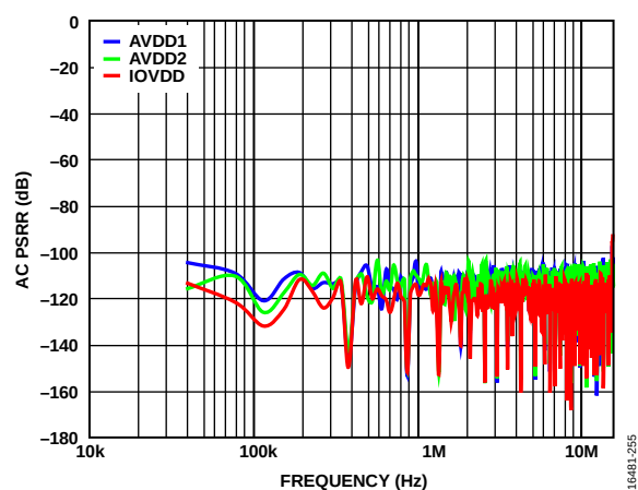
Figure 55. AC PSRR vs. Frequency, Fast Power Mode, V_{IN} = 0.1\text{ V p-p}
