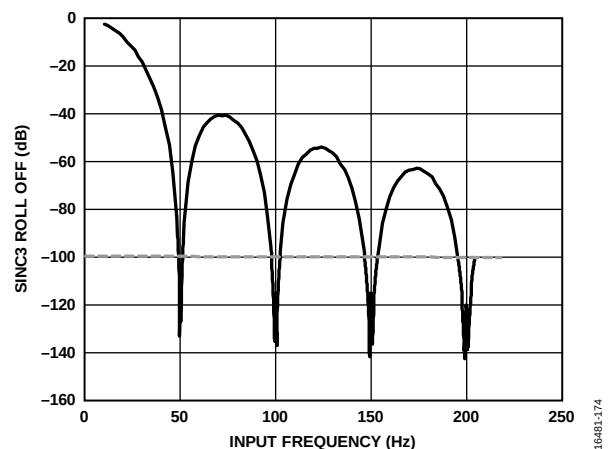
Figure 72. Sinc3 Filter Frequency Response Showing 50 Hz Rejection, 50 Hz ODR, x163,840 Decimation
