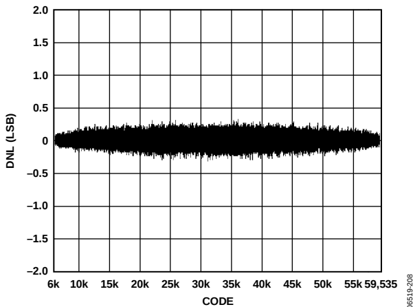
Figure 20. DNL Plot
