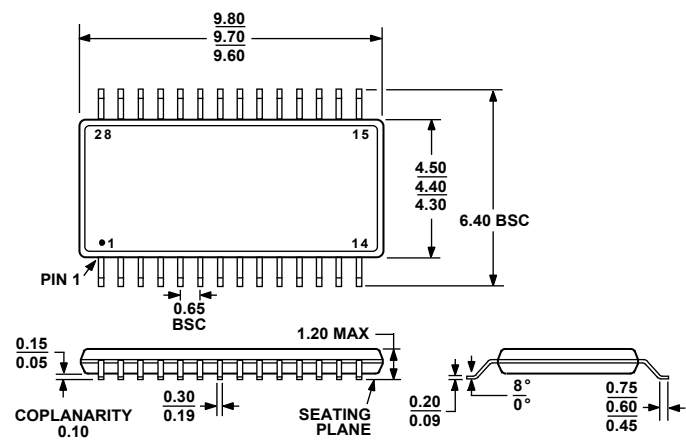
COMPLIANT TO JEDEC STANDARDS MO-153-AE Figure 56. 28-Lead Thin Shrink Small Outline [TSSOP] (RU-28) Dimensions shown in millimeters
