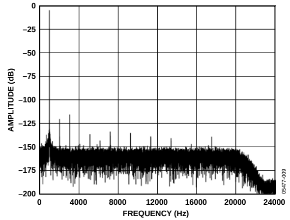
Figure 8. Low Power FFT, 1 kHz, -0.5 dB Input Tone, 256× Decimation
