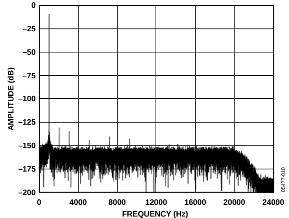
Figure 9. Low Power FFT, 1 kHz, -6 dB Input Tone, 256× Decimation
