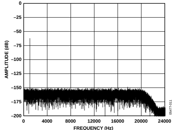
Figure 10. Low Power FFT, 1 kHz, -60 dB Input Tone, 256× Decimation
