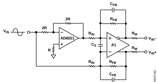
Figure 27. Single-Ended-to-Differential Conversion
