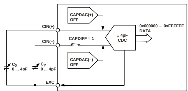
Figure 33. CDC Differential Input Mode
