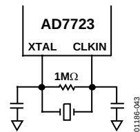
Figure 43. Crystal Oscillator Connection
