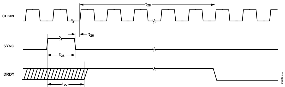
Figure 10. SYNC Timing
