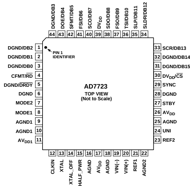
Figure 11. 44-Lead MQFP
