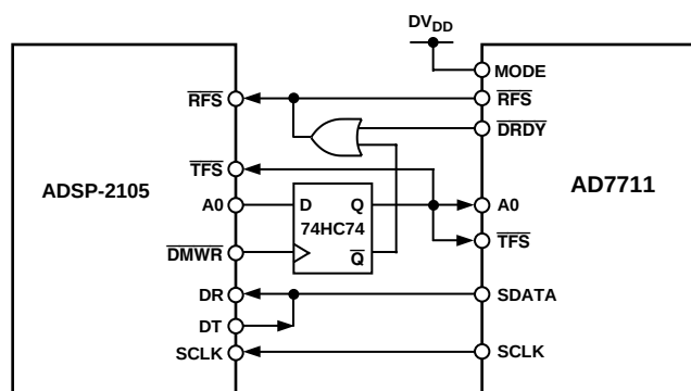
Figure 19. AD7711 to ADSP-2105 Interface
