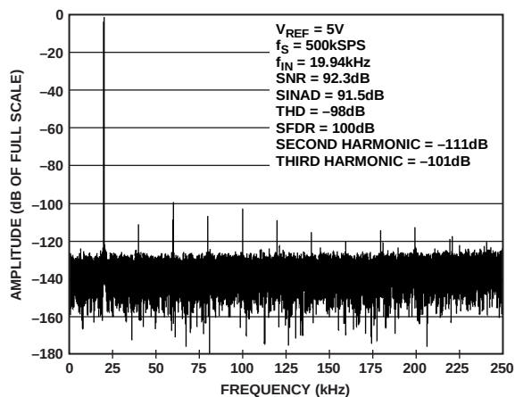
Figure 8. 20 kHz FFT, VREF = 5 V
