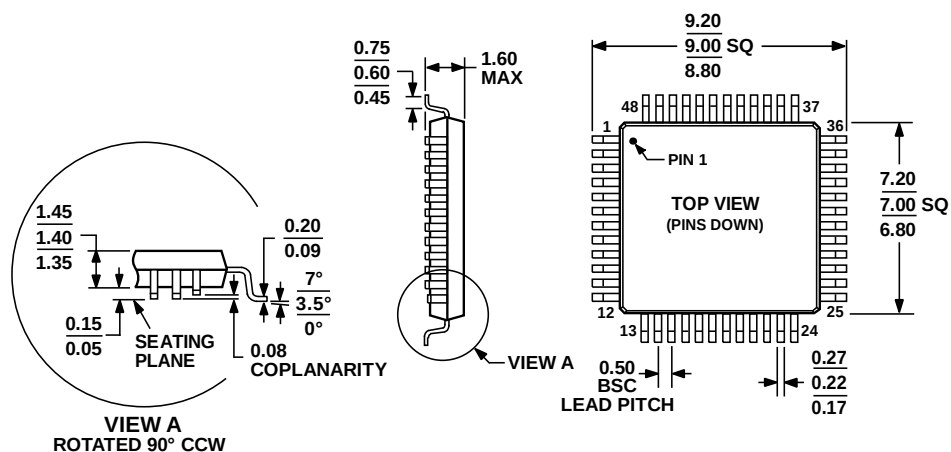
Figure 40. 48-Lead Plastic Quad Flat Package [LQFP]
