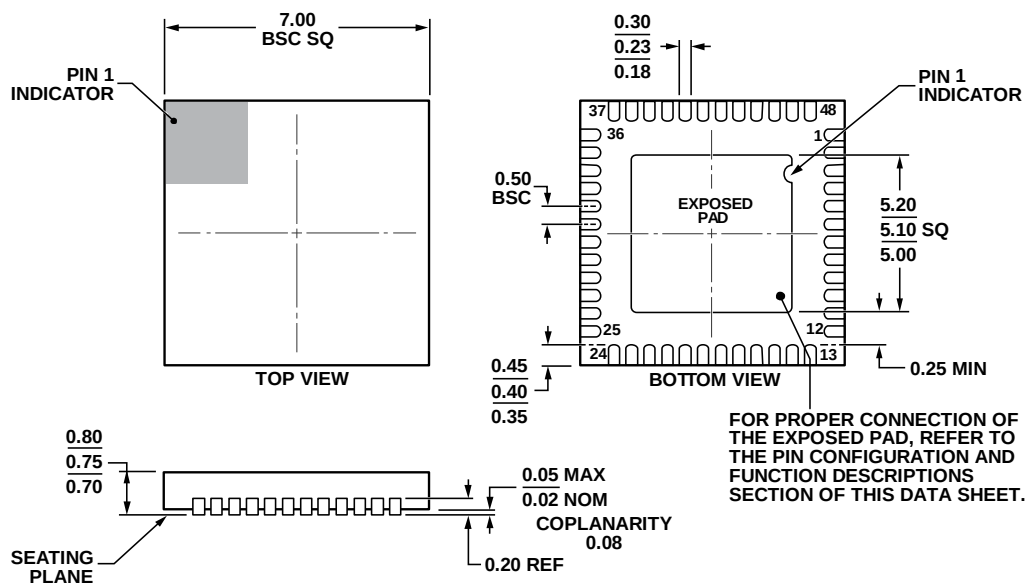
Figure 41. 48-Lead Lead Frame Chip Scale Package [LFCSP]
