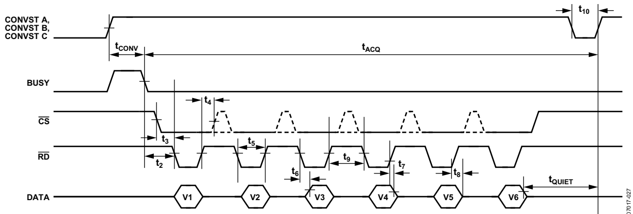
图29. 并行接口时序图( \overline{\text{W}}/\text{B} = 0 )
