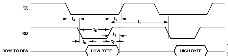
图30. 并行接口—字节操作模式的读取周期 ( \overline{\text{W}}/\text{B} = 1 , \text{HBEN} = 0 )
