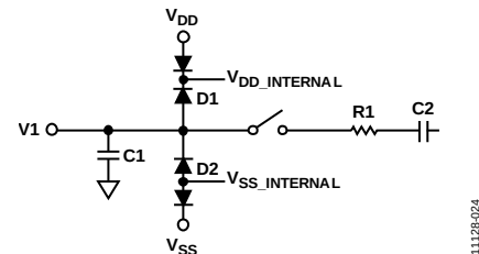
Figure 21. Equivalent Analog Input Structure
