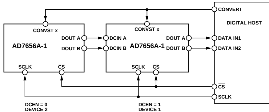
Figure 31. Daisy-Chain Configuration
