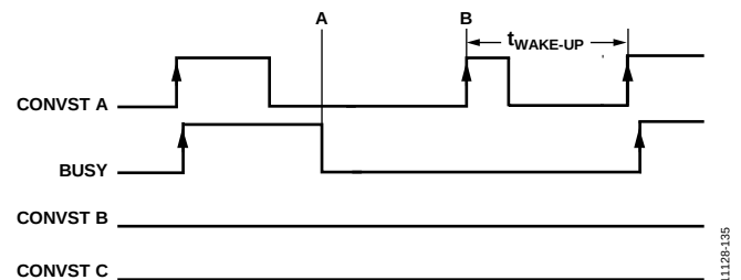
Figure 34. Entering and Exiting Partial Power-Down Mode
