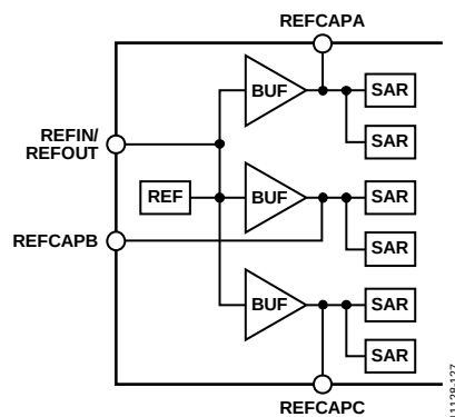
Figure 23. Reference Circuit
