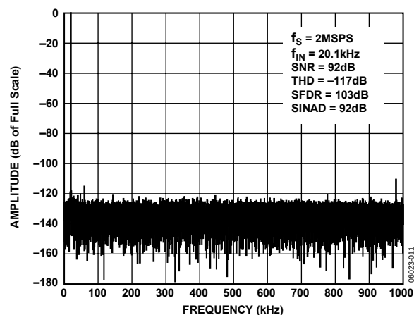
Figure 12. FFT 20 kHz
