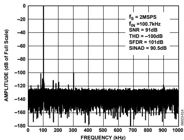
Figure 15. FFT 100 kHz
