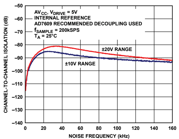
Figure 25. Channel-to-Channel Isolation
