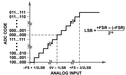
Figure 37. AD7609 Transfer Characteristic
