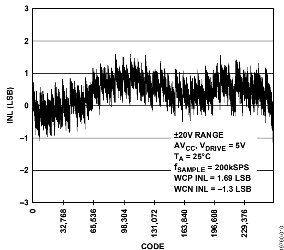
Figure 11. Typical INL, \pm 20V Range
