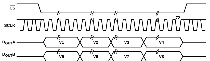
Figure 43. AD7608 Serial Interface with two DOUT Lines
