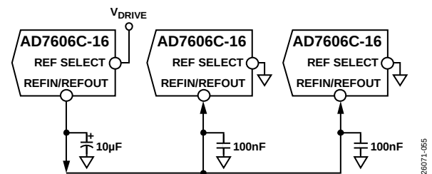
Figure 85. Internal Reference Driving Multiple AD7606C-16 REFIN/REFOUT Pins
