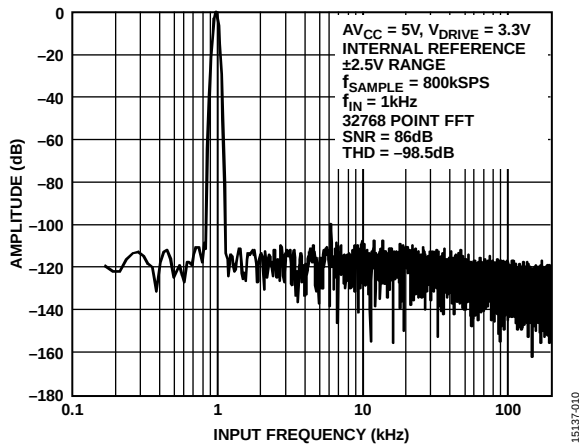
Figure 10. FFT, \pm 2.5 V Range
