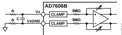
Figure 45. Input Resistance Matching on the Analog Input of the AD7606B
