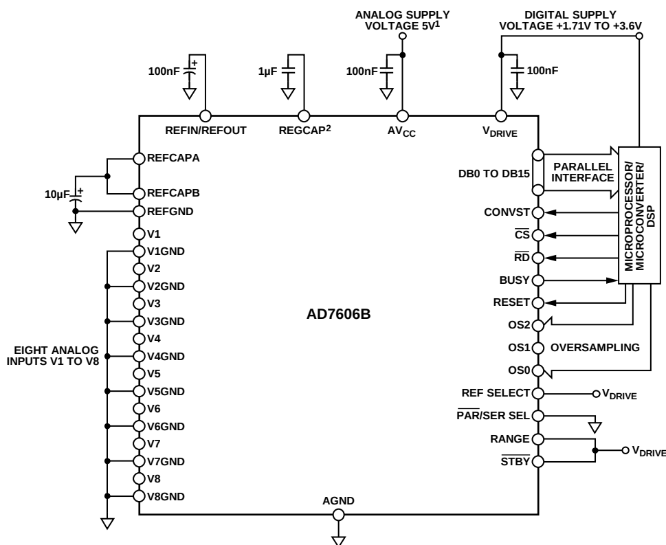
Figure 83. AD7606B Typical Connection Diagram, Hardware Mode
