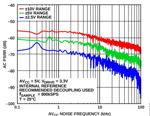
Figure 32. AC PSRR
