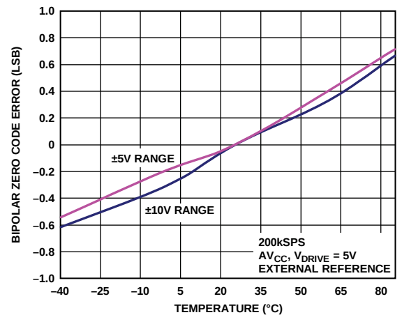
Figure 19. Bipolar Zero Code Error vs. Temperature
