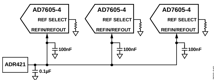
Figure 35. Single External Reference Driving Multiple AD7605-4 REFIN/REFOUT Pins
