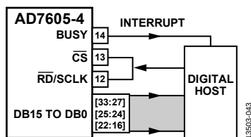
Figure 39. AD7605-4 Interface Diagram—One AD7605-4 Device Using the Parallel Bus, with \overline{CS} and \overline{RD/SCLK} Shorted Together
