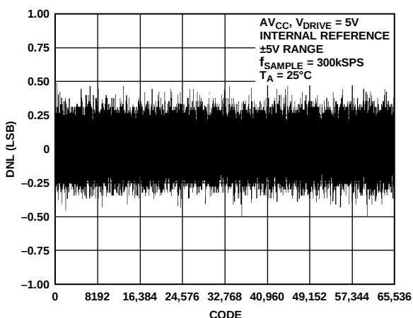
Figure 14. Typical DNL, \pm 5\text{ V} Range
