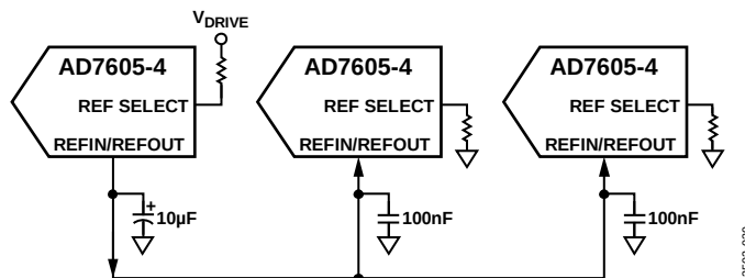
Figure 36. Internal Reference Driving Multiple AD7605-4 REFIN/REFOUT Pins
