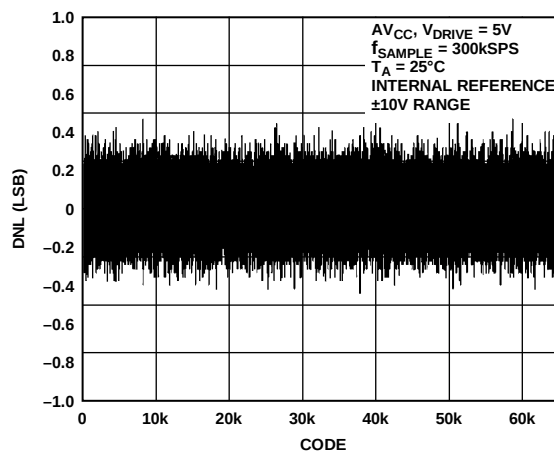
Figure 12. Typical DNL, \pm 10\text{ V} Range
