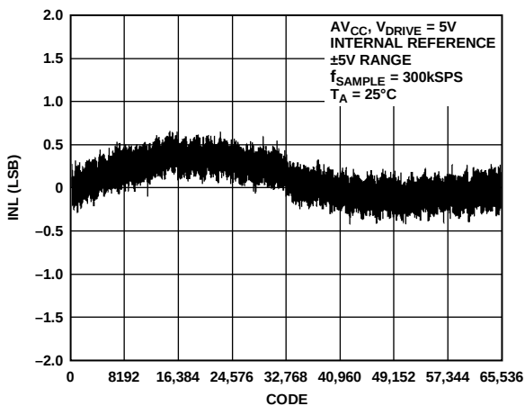
Figure 13. Typical INL, \pm 5\text{ V} Range
