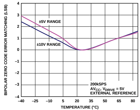
Figure 20. Bipolar Zero Code Error Matching Between Channels
