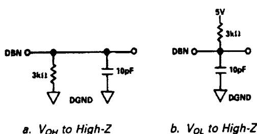
Figure 2. Load Circuits for Output Float Delay
