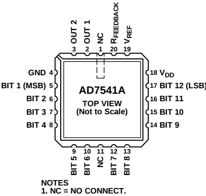
Figure 3. 20-Lead PLCC Pin Configuration
