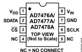
Figure 6. 8-Lead MSOP Pin Configuration
