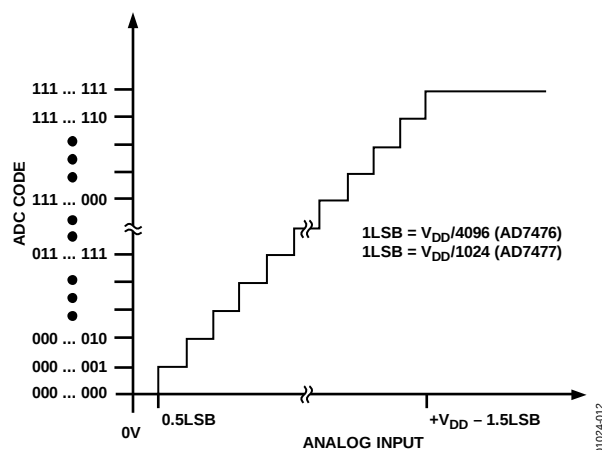
Figure 12. Transfer Characteristic for the AD7476/AD7477
