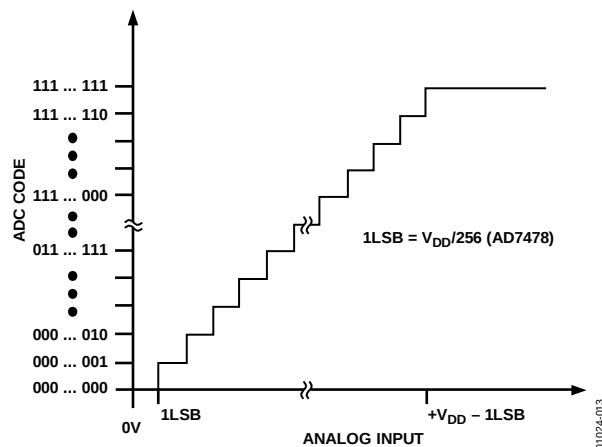
Figure 13. Transfer Characteristic for AD7478
